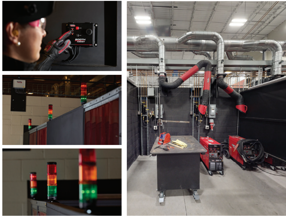
Figure 2-4B: The ideal welding booth should be 8 ft (2.4 m) x 8 ft (2.4 m) with access to essential power, tools, table and exhaust removal. Lincoln Electric's Booth Assist is a visual monitoring system for instructor
