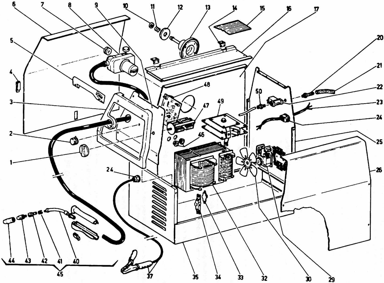
M12184, 83-318, MB135 (Mig 115)
