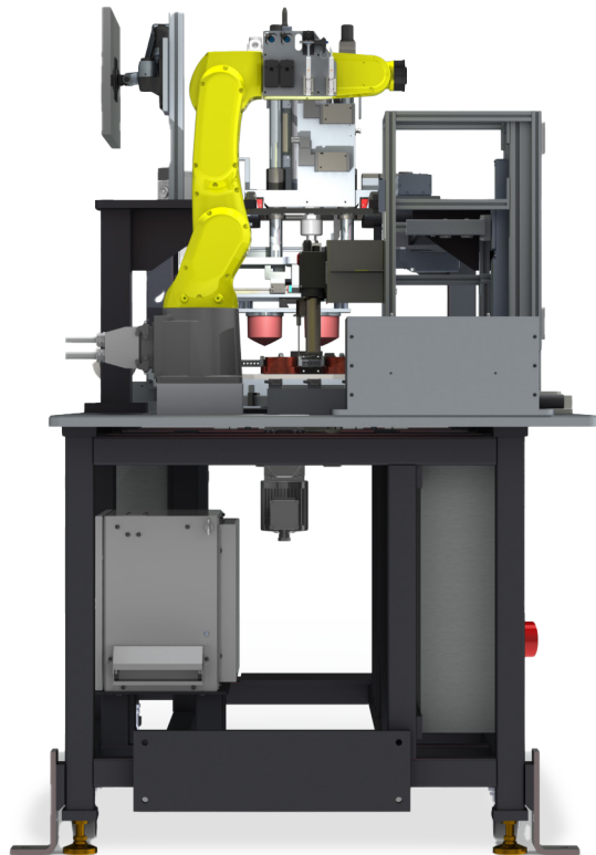
Guarding removed to show system
