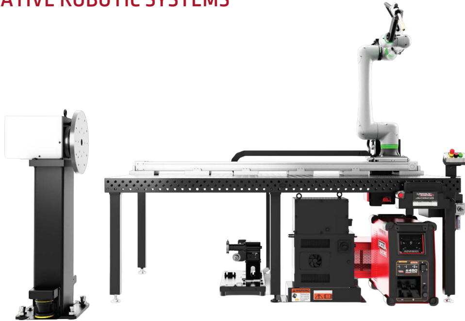
Cooper Adapt Water-Cooled Welding Cobot with Optional Rotary Positioner
