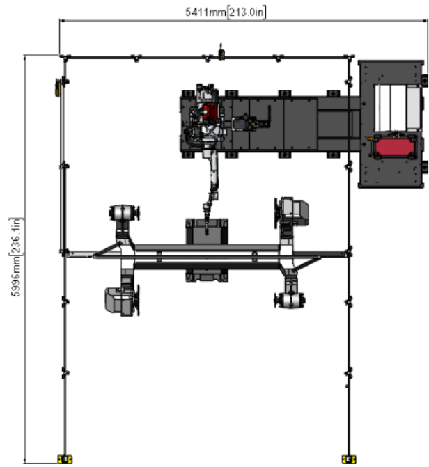
Fab-Pak XHS-RM 2000mm system with ABB robot
