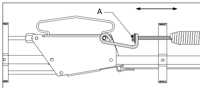
Fig. 6.4 Middenscharnier – LFA 3.1 | LFA 4.1
