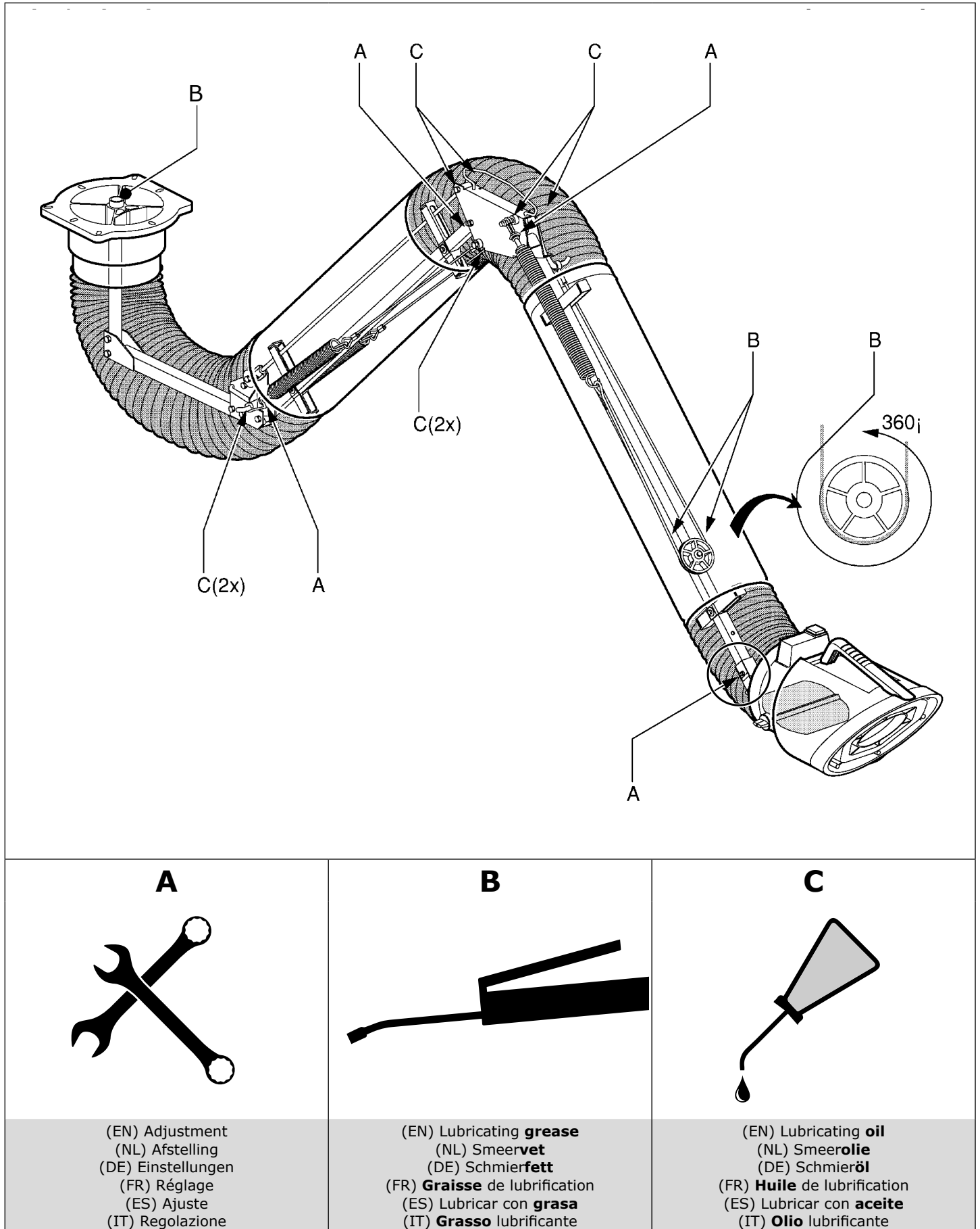
Fig. V Maintenance points LFA 3.1 | LFA 4.1
