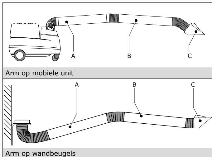
Fig. 6.1 Arm in horizontale positie
