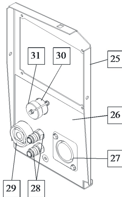
Figure B: Front Panel
