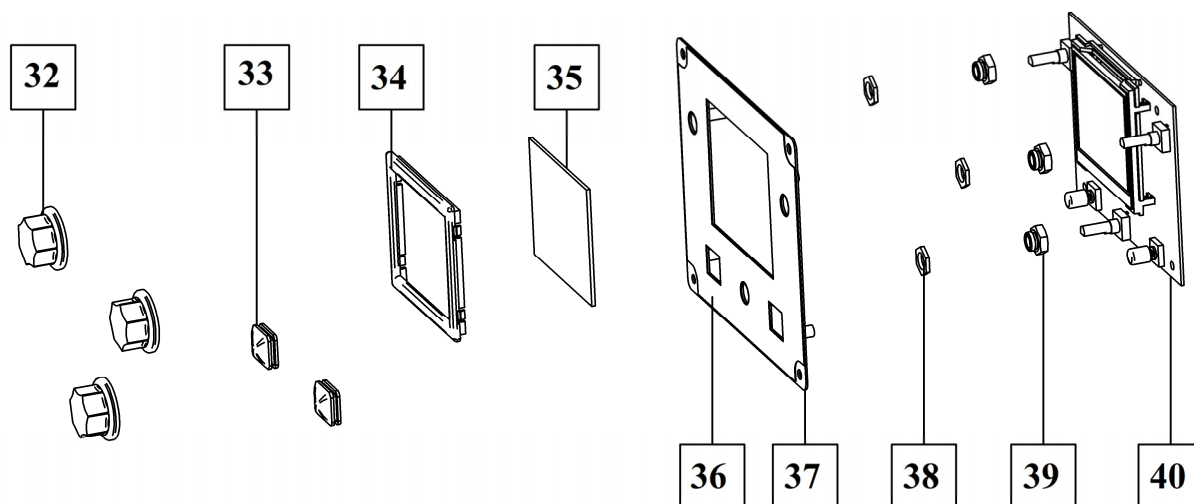
Figure C: User Interface Assembly
