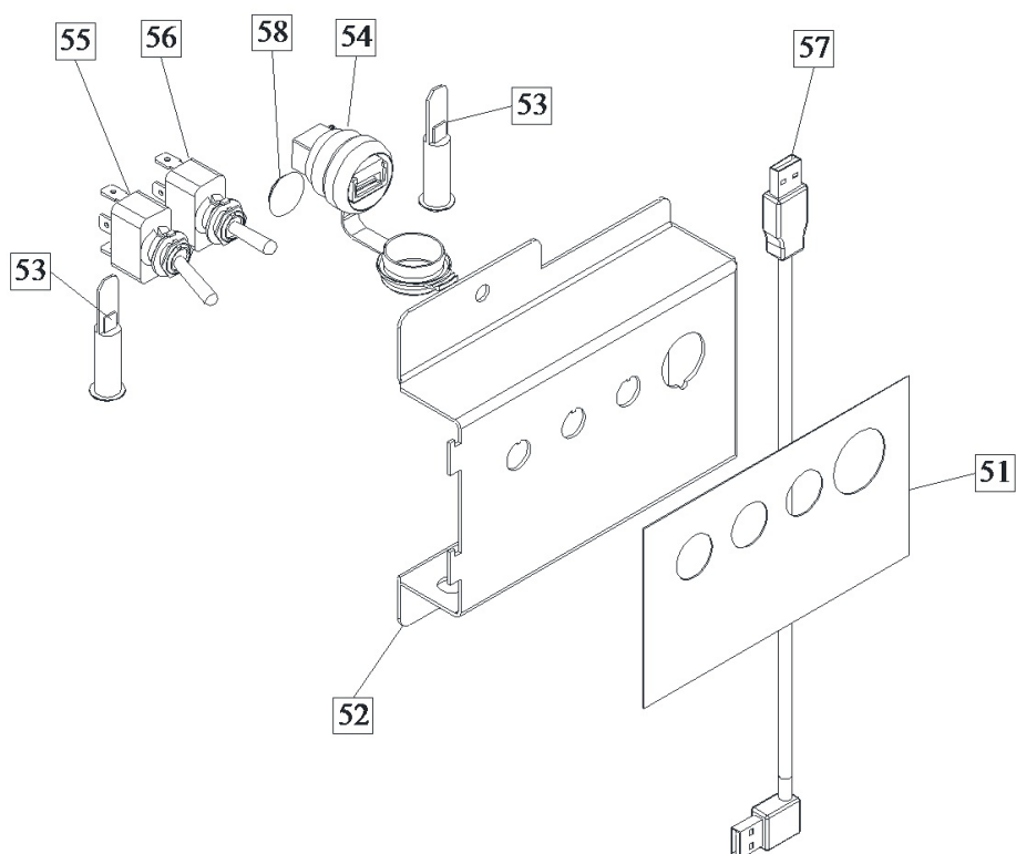
Figure E: Panel USB Divider Assembly.
