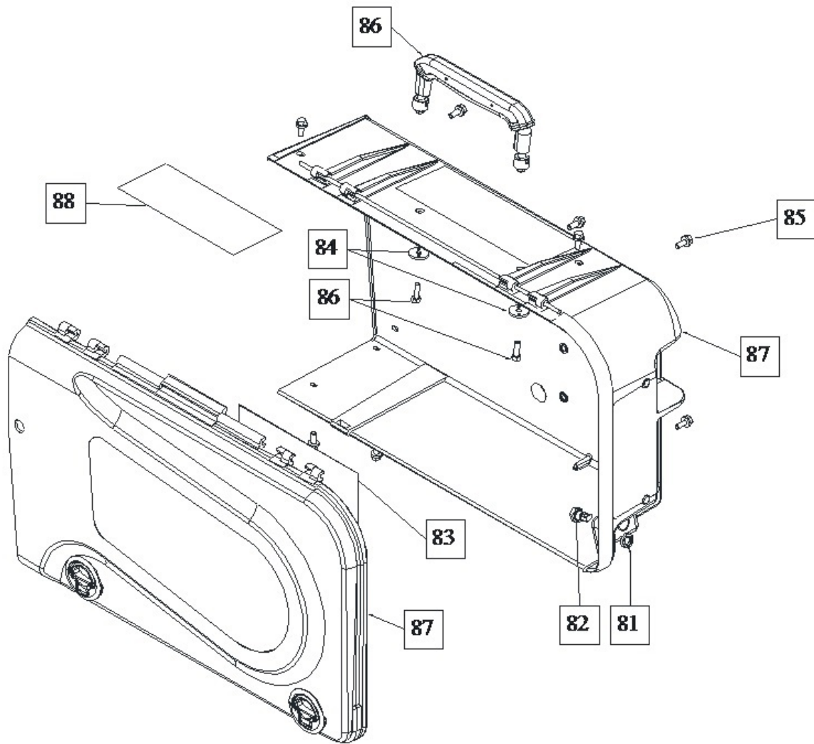
Figure G: Plastic Case
