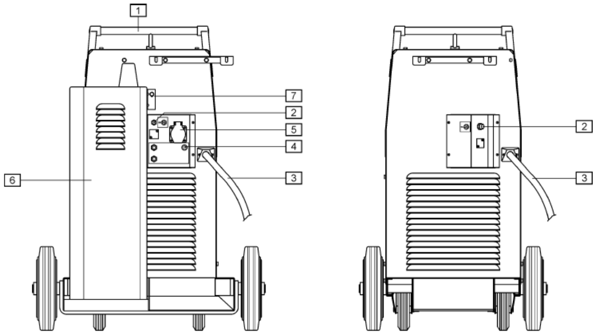
FIGURE B: Machine assembly (rear side)
