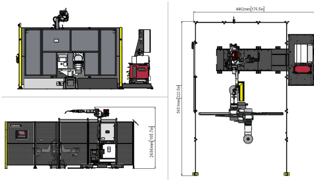
Fab-Pak XSH system 250 with ABB robot
