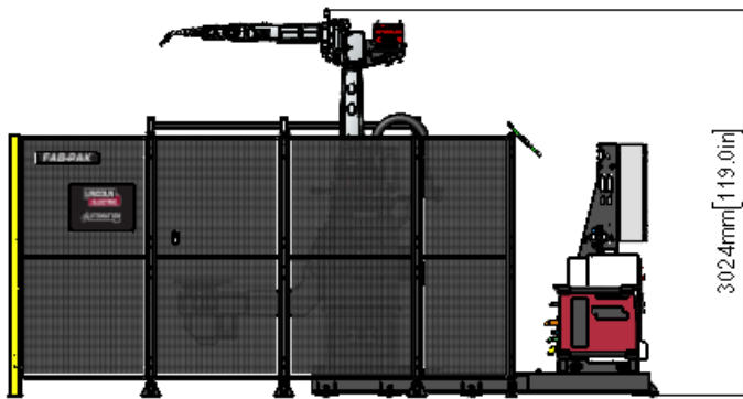
Fab-Pak ISH 750 system with ABB robot
