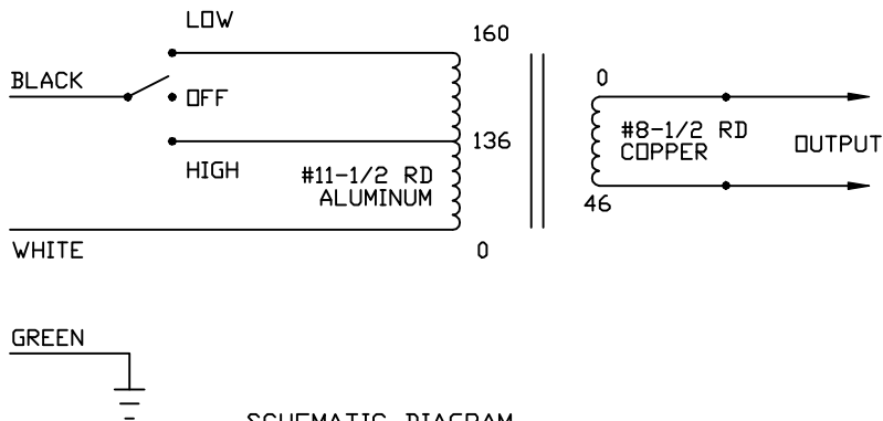
SCHEMATIC DIAGRAM
