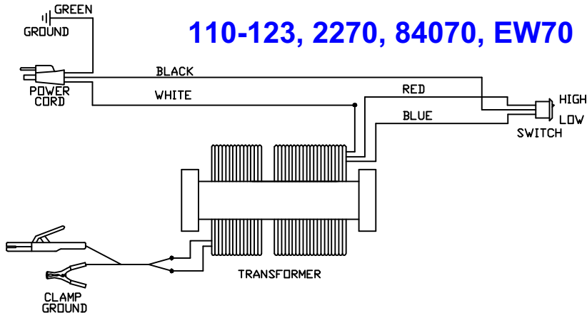
WIRING DIAGRAM
