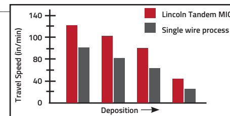
Travel speed is significantly higher with Tandem MIG vs. single-wire welding.
