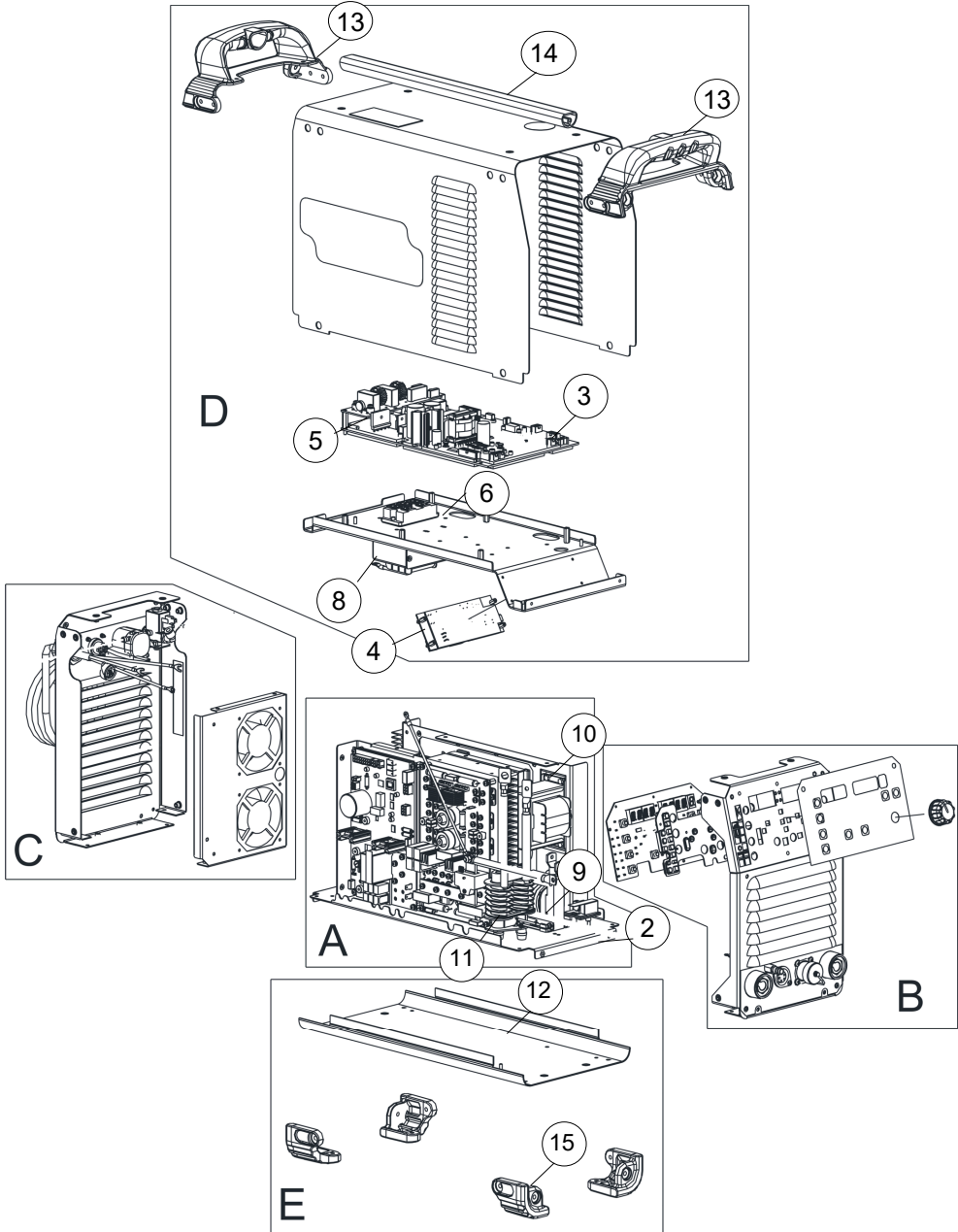
Figure A PRESTOTIG 200 CE AC/DC
