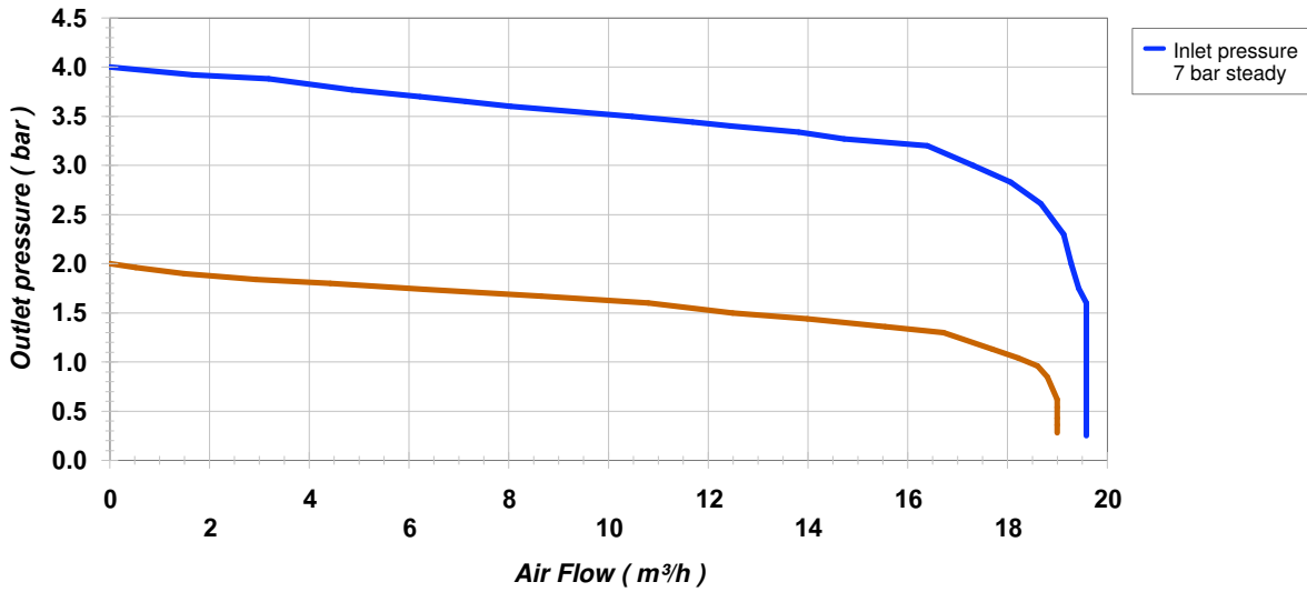
REGULATOR FLOW CURVE 818 4 bar LPG
