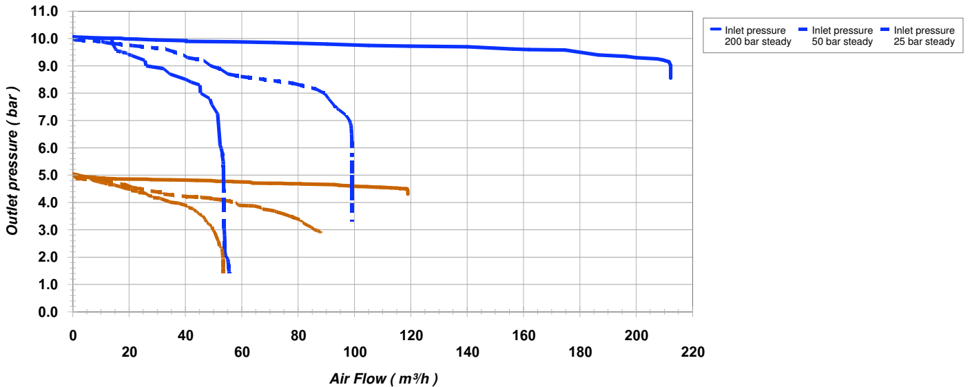
REGULATOR FLOW CURVE 818 10 bar
