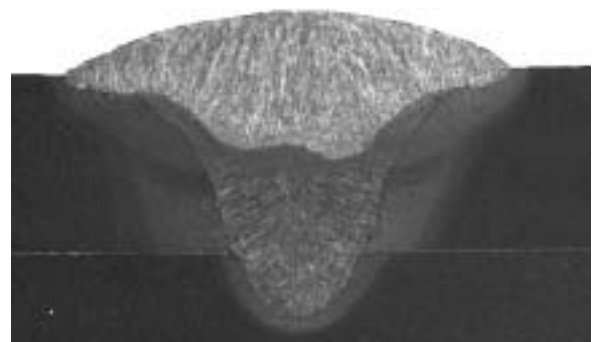
2 Pass "J" Groove
