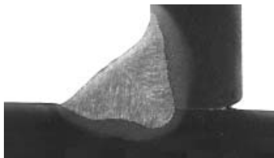
6mm Horizontal Fillet
