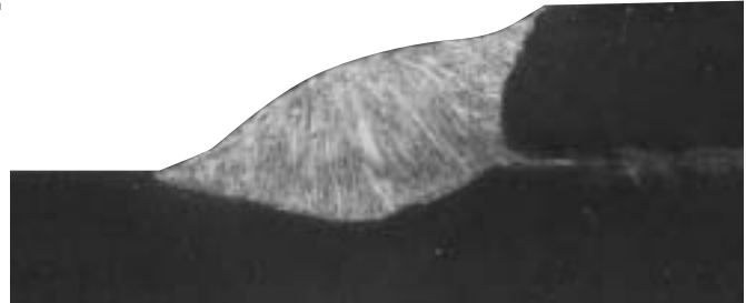
12 Gauge Lap Weld at 120 ipm travel
