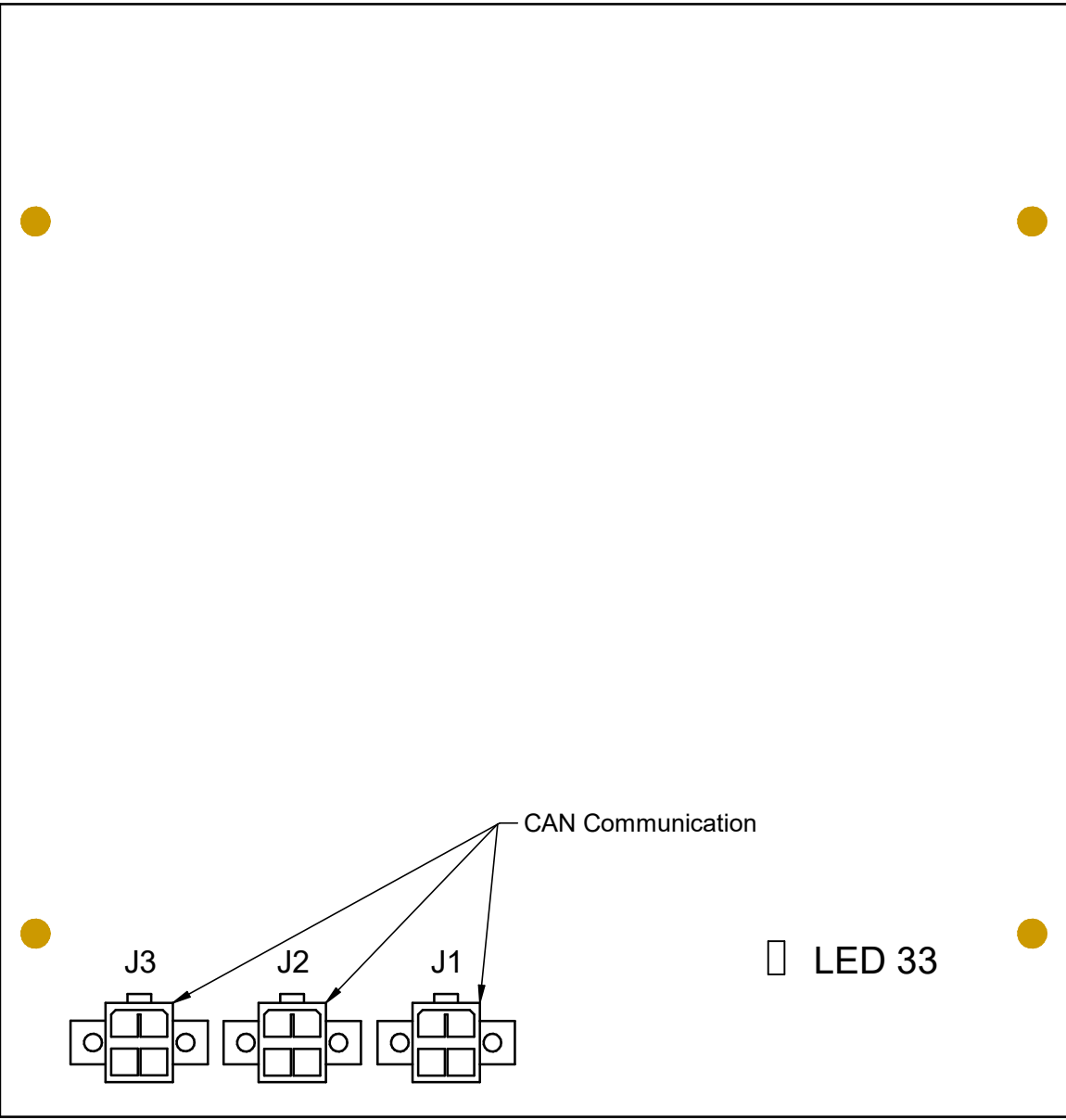
OPPOSITE COMPONENT SIDE LED 33: +15 V PRESENT
