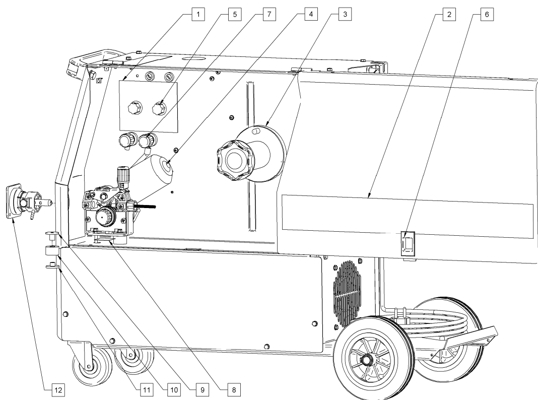
Figure C: Machine Assembly (Wire feed chamber)
