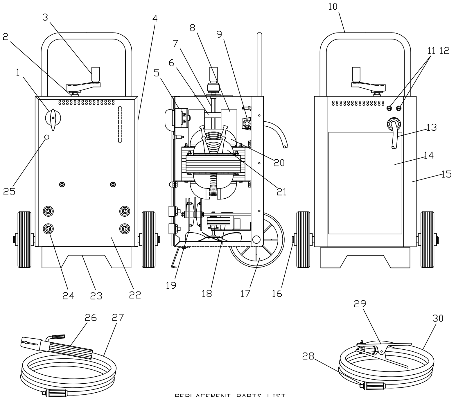
REPLACEMENT PARTS LIST 235 AMP AC/DC ARC WELDER MODEL 84241 (110-132)
