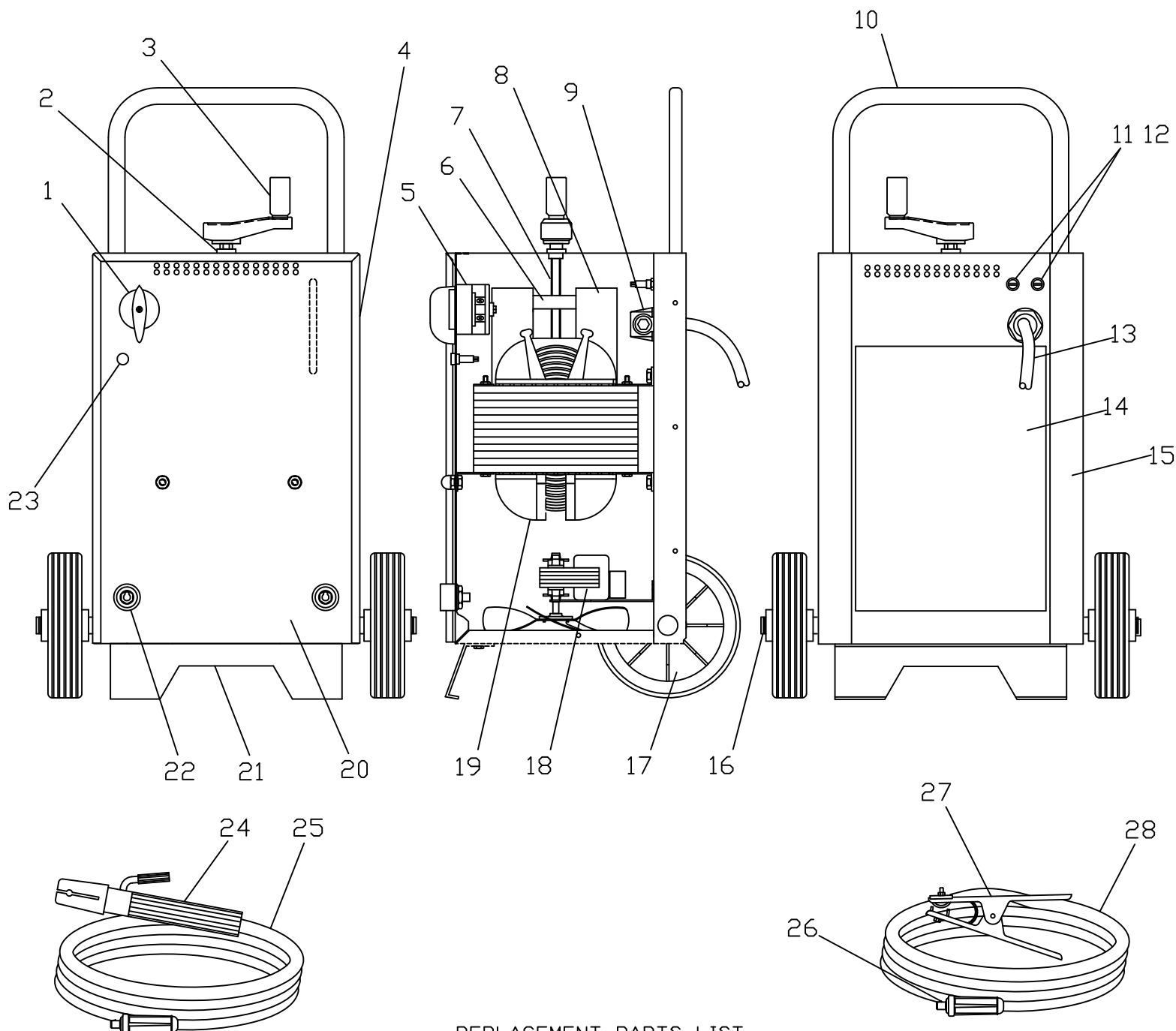
REPLACEMENT PARTS LIST 235 AMP AC ARC WELDER MODEL 84240 (110-131)
