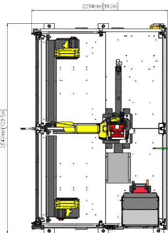
Fab-Pak CDZ-FT with FANUC robot
