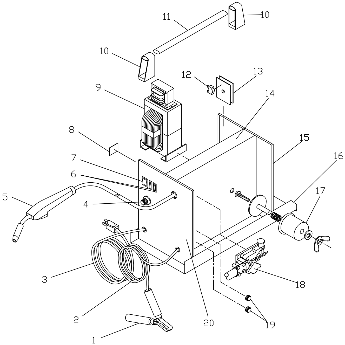
REPLACEMENT PARTS LIST 117-086, 83095, 83096, P3095, 20676 90A MIG WELDER MODEL 83095 & 83096 (117-086)
