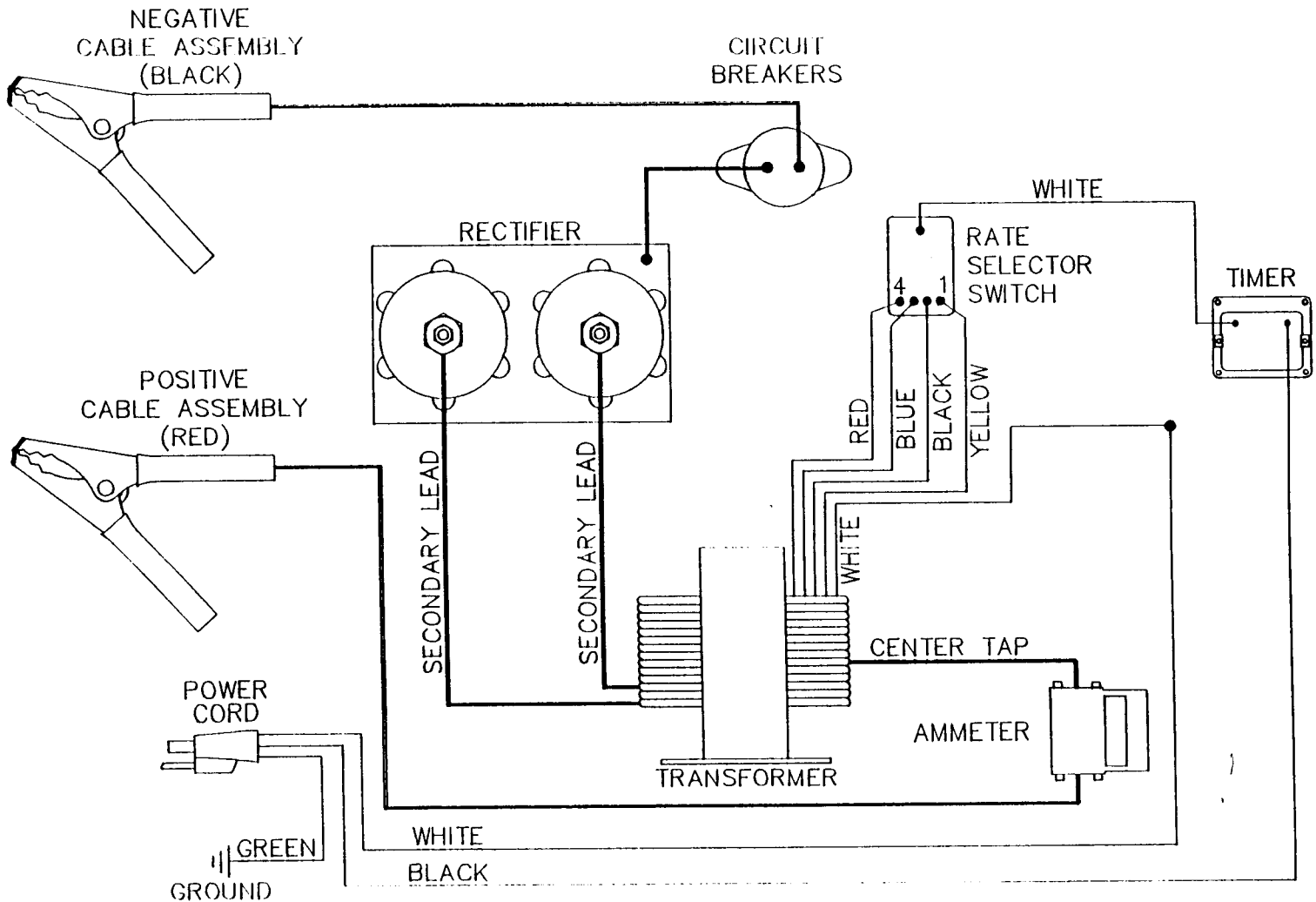
WIRING DIAGRAM
