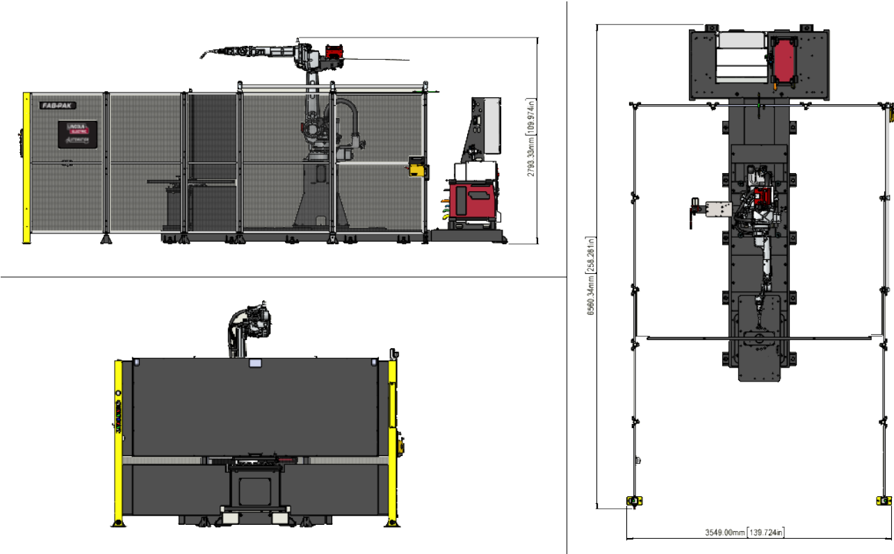
Fab-Pak XFT 3000mm system with ABB robot
